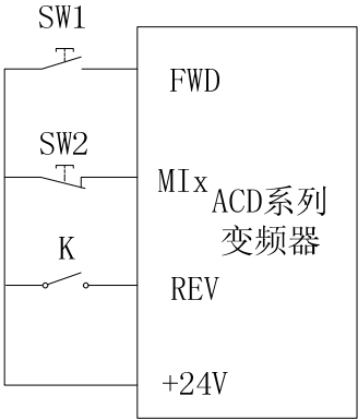
(2) 输入信号为PNP时
