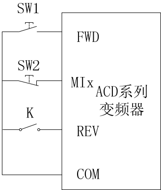
(1) 输入信号为NPN时
